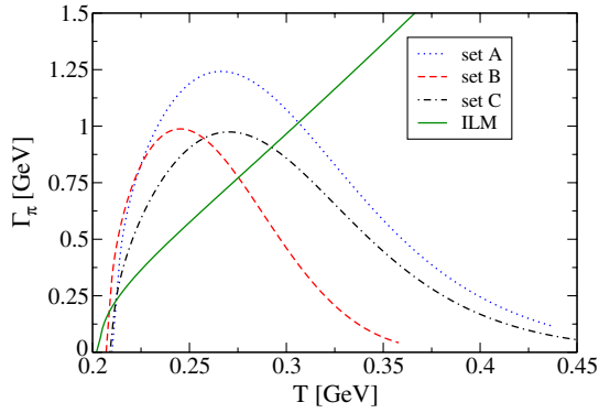
FIG. 7 (color online). The figure displays the approximate pion widths calculated from Eqs. (61) for sets A–C and the ILM.
