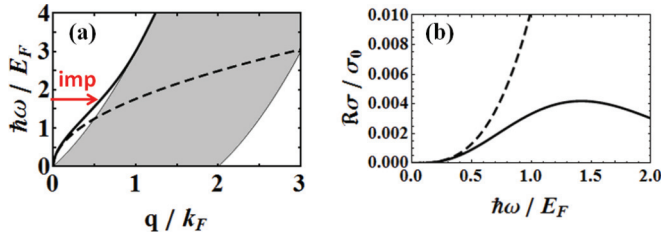
FIG. 1. (Color online) Plasmon dispersion and optical conductivity for metallic monolayers. In plot (a) we show the plasmon dispersion relation within the random phase approximation (solid line) and within the Drude model, i.e., in the small frequency limit (dashed line). The gray area denotes the regime of single-particle excitations. Random assembly of impurities breaks the translation invariance, which allows a zero-momentum photon to couple to a finite-momentum plasmon (sketched by the red arrow). In plot (b) we show the optical absorption for the plasmon emission process through impurity scattering. We plot the real part of the conductivity in units of \sigma_0 = \frac{e^2}{4\hbar} vs photon energy in units of Fermi energy E_F . One can see that the small frequency limit (dashed line) significantly overestimates the more exact RPA result (solid line).
