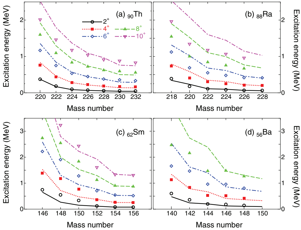
FIG. 11. (Color online) Excitation energies of low-lying yrast positive-parity collective states of {}^{220-232}\text{Th} , {}^{218-228}\text{Ra} , {}^{146-156}\text{Sm} , and {}^{140-150}\text{Ba} , as functions of the mass number. In each panel lines and symbols denote the theoretical and experimental [64] values, respectively. Figure legends are found in (a).
