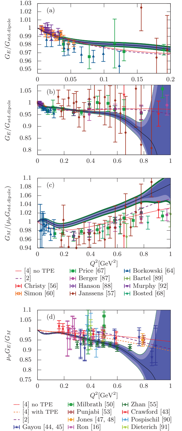
FIG. 10. (Color) The form factors G_E and G_M , normalized to the standard dipole, and G_E/G_M as a function of Q^2 . Black line: Best fit to the new Mainz data; blue area: statistical 68% pointwise confidence band; light blue area: experimental systematic error; green outer band: variation of the Coulomb correction by \pm 50\% . The different data points depict the previous measurements [2,4,43–45,47,48,50,53,55–57,60,67,68,87–91] as in Refs. [2,4] with the data points of Refs. [16,64,92] added.
