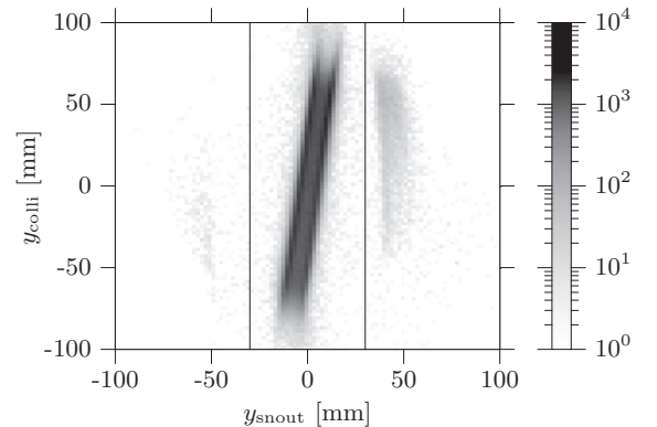
FIG. 6. Histogram of y_{\text{colli}} versus y_{\text{snout}} of the measurement with spectrometer B at 32.5^\circ at an incident energy E = 180 MeV. The events around y_{\text{snout}} = 0 correspond to good events, and the sidebands result from back scattering from the snout walls. The black vertical lines indicate the cut used in the analysis. The gray scale is logarithmic to emphasize the events in the left and right sideband. The diagonal ridges seen in the good events are caused by scattering off the target walls.
