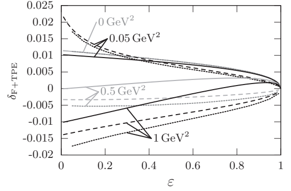
FIG. 18. Comparison of the complete TPE correction \delta_{\text{F+TPE}} (without the soft part included in Maximon-Tjon) for four different Q^2 values. Solid: Fit to data; dashed: calculation with the approximation of Ref. [96]; dotted: TPE corrections from Refs. [97–99].
