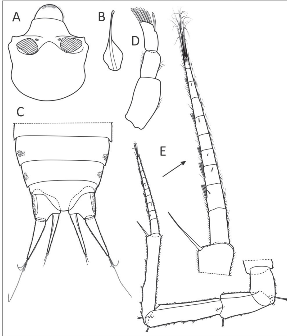
Fig. 3. Alphoniscus (Illyrionethes) iapodicus n. sp. paratype ♀: A, cephalon; paratype ♂: B, dorsal scale-sensilla; C, pleonites 4, 5, telson and uropods; D, antenna; E, antenna.
