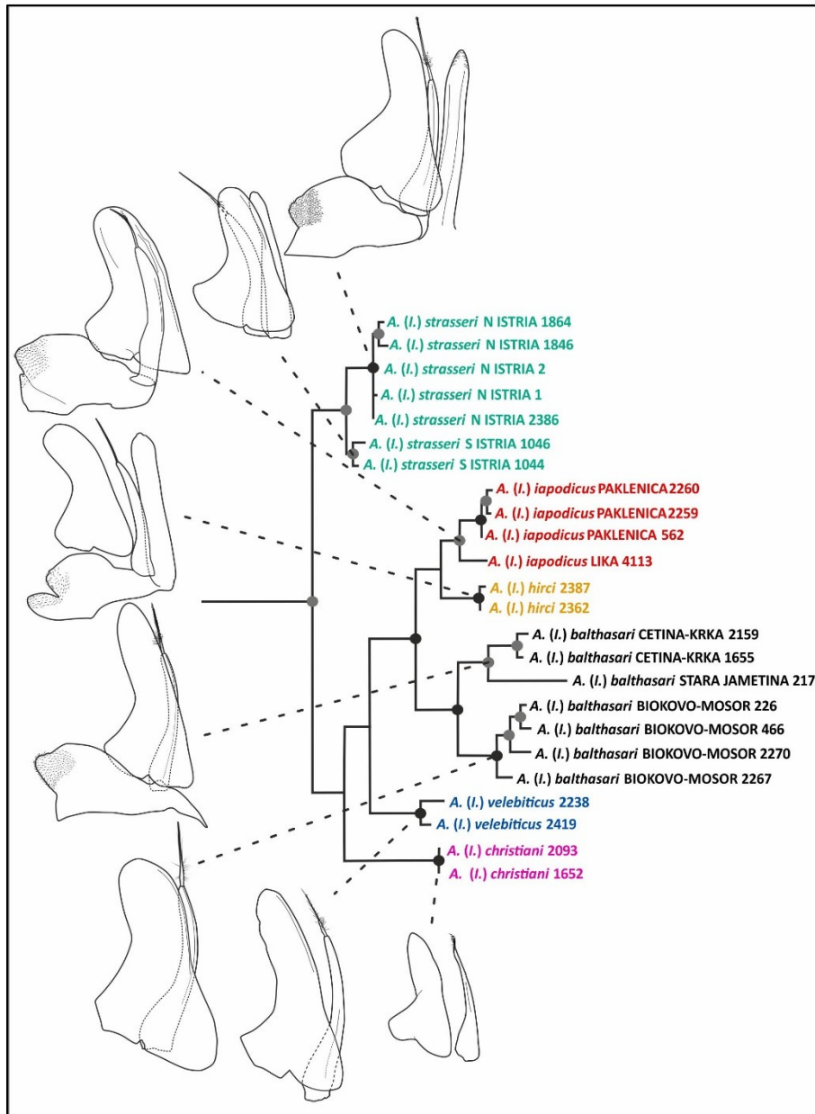
Figure 5. Alphonisus (Illyrionethes) , the strasseri -lineage. Maximum likelihood (ML) phylogenetic tree obtained by 16S data set with male pleopod 1. Black and grey dots indicate bootstrap values of \geq 0.95 and > 0.75 , respectively. Adapted from Bedek et al. 2017 and 2019c, with permission.
