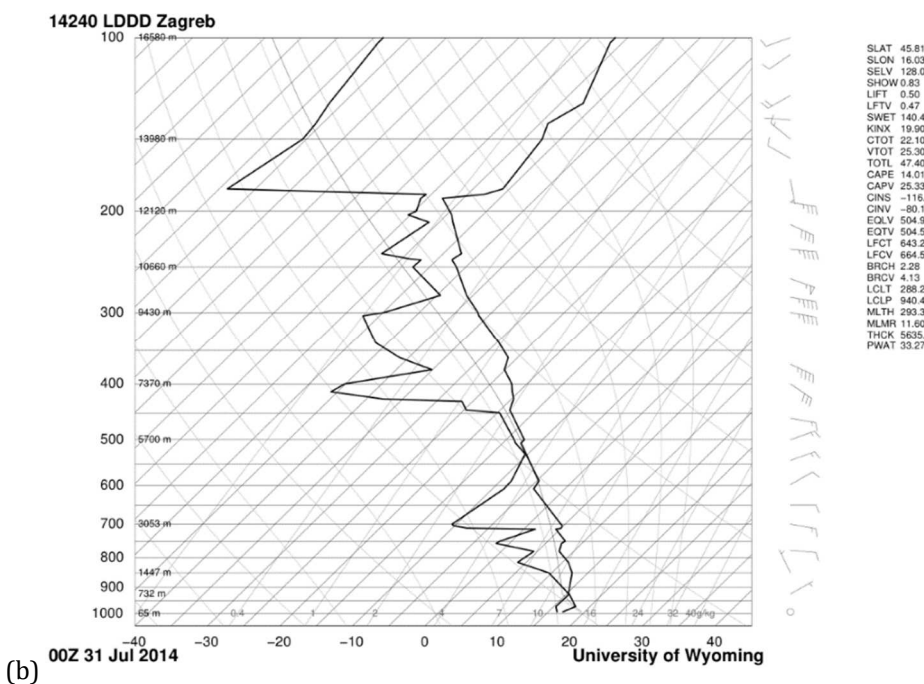
Slika 12: Termodinamički dijagram radiosondaže za postaju Zagreb – Maksimir (a) 30.07.2014. u 12:00 UTC i (b) 31.07.2014. u 00:00 UTC (izvor: http://weather.uwyo.edu/upperair/sounding.html )
