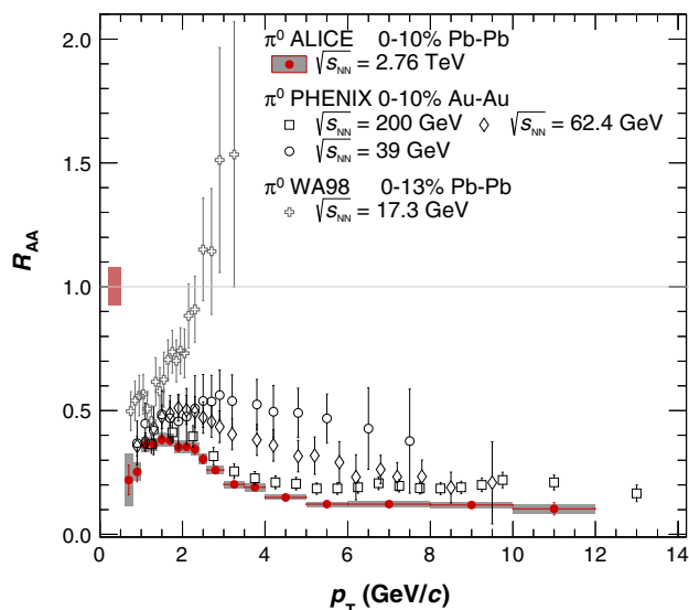
Fig. 8 (Color online) Neutral pion nuclear modification factor, R_{AA} , in Pb–Pb collisions at \sqrt{s_{NN}} = 2.76 TeV for the 0–10 % class in comparison to results at lower energies. The box around unity reflects the uncertainty of the average nuclear overlap function ( T_{AA} ) and the normalization uncertainty of the pp spectrum added in quadrature. Horizontal bars reflect the bin width. The center-of-mass energy dependence of the neutral pion R_{AA} is shown with results from Au–Au collisions at \sqrt{s_{NN}} = 39, 62.4 [34], and 200 GeV [31] as well as the result from the CERN SPS [69] (using scaled p-C data as reference) along with the results for Pb–Pb at \sqrt{s_{NN}} = 2.76 TeV. The scale uncertainties of the measurements at lower energies of the order of 10–15 % are not shown
