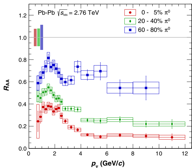
Fig. 7 (Color online) Neutral pion nuclear modification factor R_{AA} for three different centralities (0–5, 20–40, 60–80 %) in Pb–Pb collisions at \sqrt{s_{NN}} = 2.76 TeV. Vertical error bars reflect statistical uncertainties, boxes systematic uncertainties. Horizontal bars reflect the bin width. The boxes around unity reflect the uncertainty of the average nuclear overlap function ( T_{AA} ) and the normalization uncertainty of the pp spectrum added in quadrature
