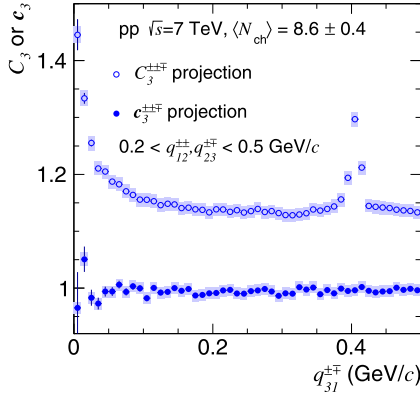
Fig. 1. Demonstration of the removal of the K_s^0 decay from three-pion cumulants. Mixed-charge three-pion correlations are projected against the relative momentum of a mixed-charge pair ( q_{31}^{+-} ). The K_s^0 decay into a \pi^+ + \pi^- pair is visible as expected around 0.4 GeV/c. The FSI enhancement of the mixed-charge pair “31” is also visible at low q_{31}^{+-} . FSI corrections are not applied. Systematic uncertainties are shown by shaded boxes.
