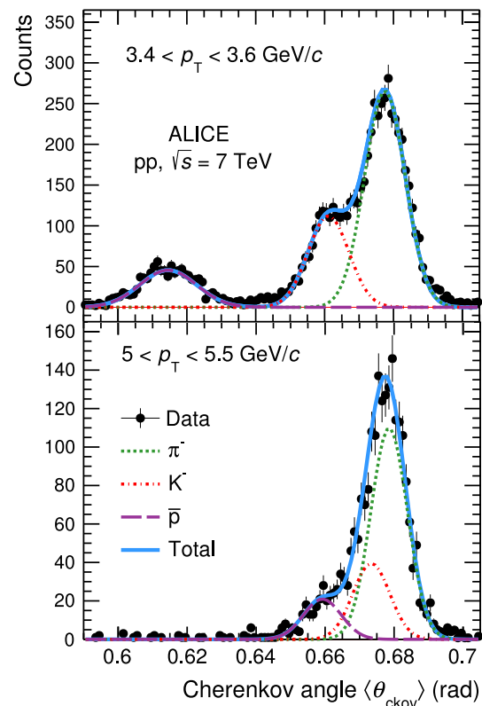
Fig. 7 Distributions of \langle\theta_{\text{ckov}}\rangle measured with the HMPID in the two narrow p_T intervals 3.4 < p_T < 3.6 GeV/c ( top ) and 5 < p_T < 5.5 GeV/c ( bottom ) for tracks from negatively charged particles. Solid lines represent the total fit (sum of three Gaussian functions). Dotted lines correspond to pion, kaon and proton signals. The background is negligible
