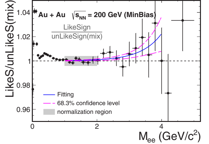
FIG. 18. (Color online) Ratio of the same-event like-sign to the mixed-event unlike-sign distributions. The gray area indicates the normalization region. The solid and dashed lines depict an empirical fit to the distribution in the mass region of 1–4 \text{GeV}/c^2 and the fit uncertainties, respectively.
