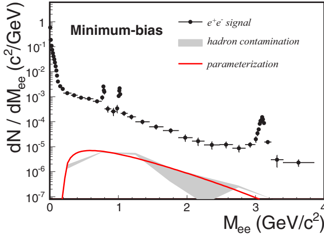
FIG. 26. (Color online) Estimated hadron contamination from e - h and h - h contributions owing to the finite contaminated hadrons in the electron sample compare to the e^+e^- pair signal in 200-GeV Au + Au collisions.
