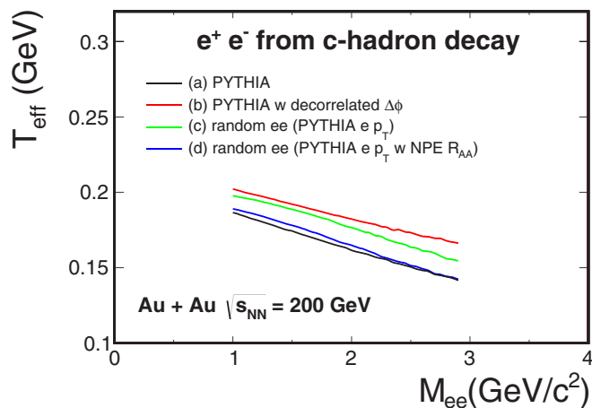
FIG. 38. (Color online) Slope parameters T_{\text{eff}} versus invariant mass for dielectrons from charmed hadron decays. Different lines show the outcome from PYTHIA calculations assuming different levels of correlations between charm pairs.
