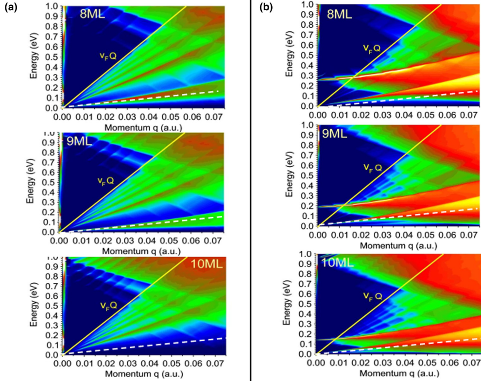
FIG. 6. (Color online) Intensities of the low-lying electronic excitations for different Ag(111) slab thicknesses (8, 9 and 10 ML) in the (a) jellium and (b) Chulkov models. The color intensity is in arbitrary units and scales linearly as 0, black; 0.2, light blue; 0.4, light green; 0.6, red; 0.8, yellow; and 1.0, white.
