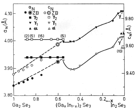
Figure 5. Phase diagram (\text{Ga}_x\text{In}_{1-x})_2\text{Se}_3 at room temperature: dependence of normalized unit cell parameters, a_N and c_N , on x . Extrapolated values of (a_N)_{\text{ZB}} and (c_N)_{\text{ZB}} , after the transition \gamma_2 \rightarrow \text{ZB} , are shown by double circles. In parentheses: molar fraction of minor phases.
