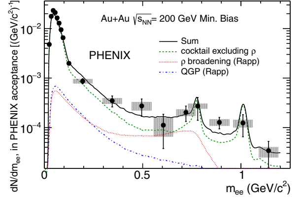
FIG. 34. MB invariant mass spectrum compared to the model calculations of Rapp (solid line) [74]. The main contributions, the in-medium \rho broadening (dotted line), the QGP thermal radiation (dot-dashed line), and the cocktail excluding the \rho (dashed line) are also shown.
