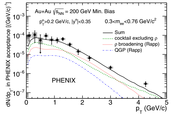
FIG. 35. Dielectron p_T distribution in the LMR compared to model calculations (solid line) [74]. The main contributions, the in-medium \rho broadening (dotted line), the QGP thermal radiation (dot-dashed line), and the cocktail excluding the \rho (dashed line) are also shown.
