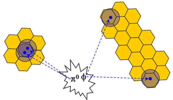
FIG. 2. Sketch illustrating the HBD response to an e^+e^- pair from \pi^0 Dalitz decay and from a \phi meson decay. The circles represent the Čerenkov blobs, whereas the hexagons are the hexagonal pads of the HBD readout plane.
