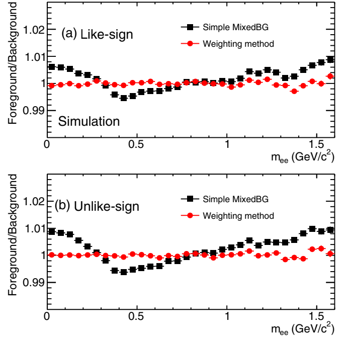
FIG. 11. Foreground to mixed-background ratio of (a) like-sign and (b) unlike-sign mass spectra ratio in a MC simulation. The foreground is generated with flow, whereas the mixed events are produced without flow, i.e., using a simple mixed-event technique (squares) and with flow modulation using the weighting method (circles).
