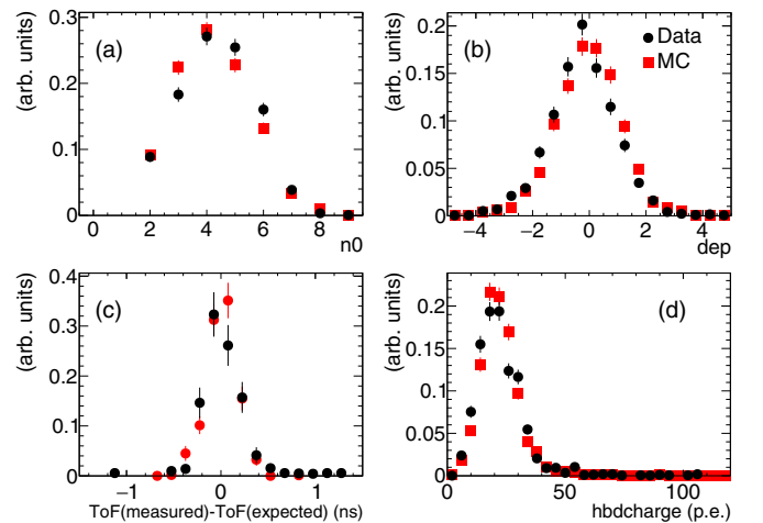
FIG. 21. Comparison of electron identification variables in data (black) and in simulations (red). The variables are described in Sec. III C. Electrons in data and simulations are from fully reconstructed \pi^0 Dalitz decays with opening angle larger than 100 mrad.
