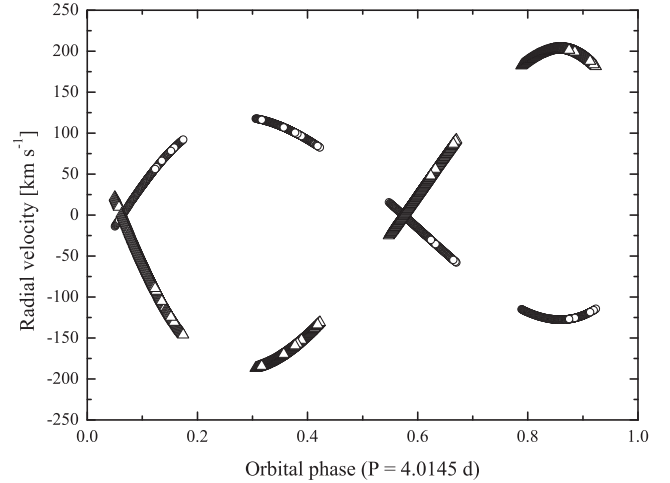
Figure 4. RVs of both binary components computed from the orbital solution reported in Table 3. The primary component is shown by open circles, whereas the secondary with open triangles.
