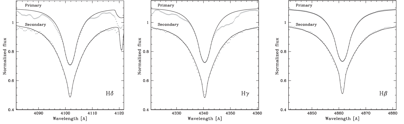
Figure 6. Best-fitting model (solid line) to the disentangled spectra (symbols) of both components of the Spica binary system. The spectrum of the primary was vertically shifted for clarity.
