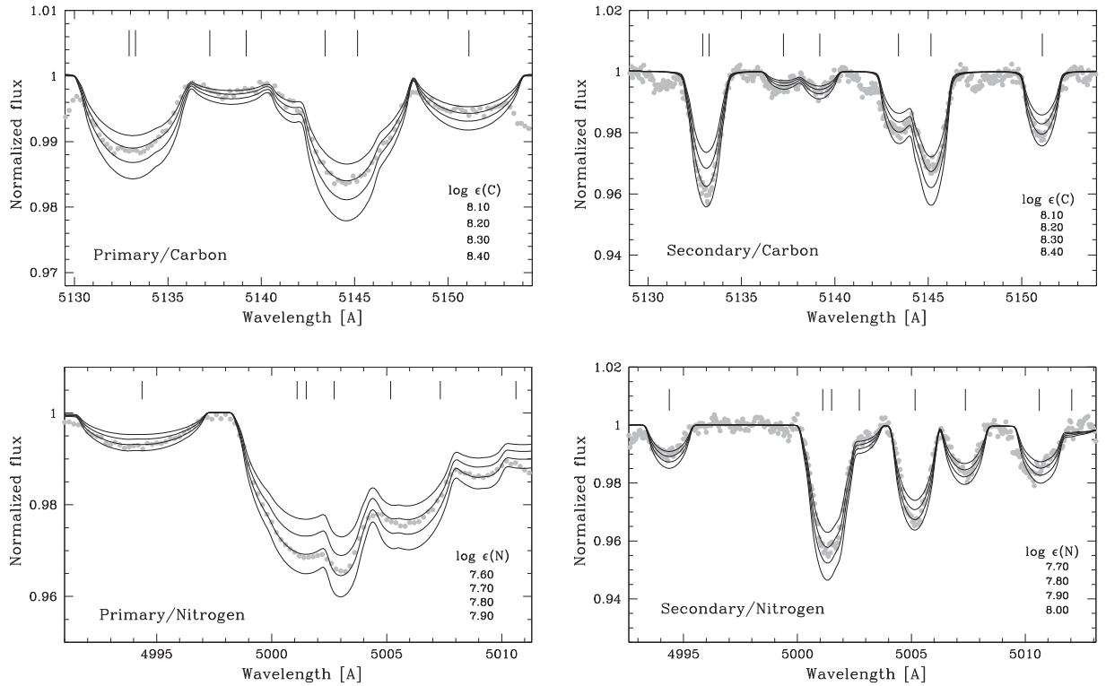
Figure 7. Fits of the theoretical spectra (lines) to the renormalized disentangled spectra of both stars (symbols) in the regions of carbon (top) and nitrogen (bottom) lines, and assuming different abundances of these elements. The columns (from left to right) refer to the primary and secondary component; the assumed abundances are indicated in the plot, where the smallest number corresponds to the weakest line. Note different X and Y scales for the primary and secondary which is due to large difference in v \sin i values of the two stars.
