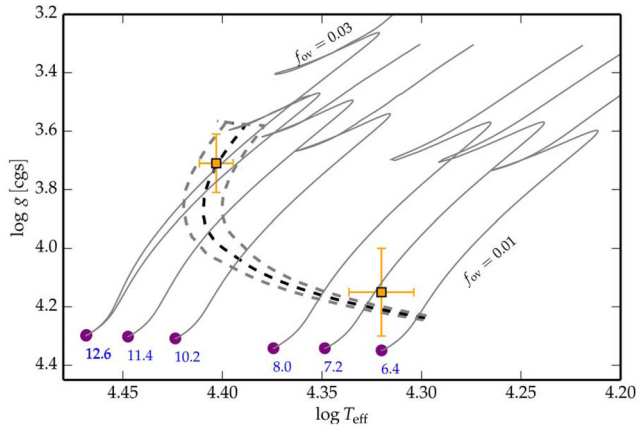
Figure 10. Location of the primary and secondary components of the Spica system in the T_{\text{eff}}\text{--}\log g Kiel diagram, along with the MESA evolutionary tracks. A track corresponding to a higher overshoot is shown for one selected mass to illustrate that it is impossible to constrain overshoot parameter f_{\text{ov}} from the models due to large error box in the determined fundamental parameters. Dashed lines show three isochrones corresponding (from bottom to top) to 11.5, 12.5, and 13.5 Myr
