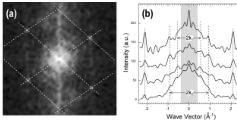
Fig. 6.40. 3 ML Ag/V(100)-(5 \times 1). (a) Fourier transform of the surface wave STM image. (b) Profile scans over the ring-like feature from several 2 ML images along the high symmetry direction.
