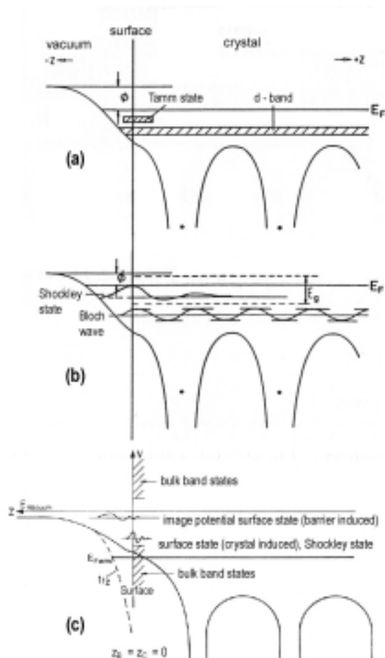
Fig. 4.1. [7] (a) A Tamm state is a split off from a band ( d -band here) of the crystal by the change of the potential at the surface. (b) A Shockley state is created in a band gap of the bulk band structure due to the termination of the crystal by a surface. (c) Distinction between the crystal (Shockley states) or barrier induced (image states) surface states.
