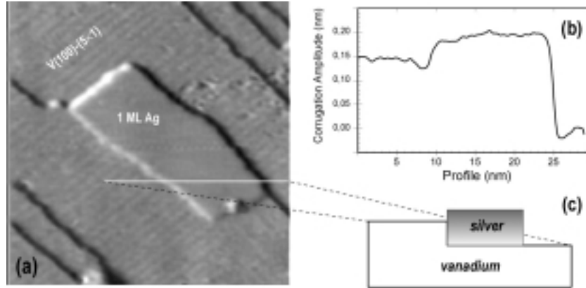
Fig. 6.8. (a) STM image of the 1 ML thick silver island. U_B = 0.45 \text{ V} , I_T = 1.2 \text{ nA} . (b) Profile scan over the 1 ML silver island as indicated by the white line. (c) Schematic of the vanadium surface and silver island along the white line in (a).
