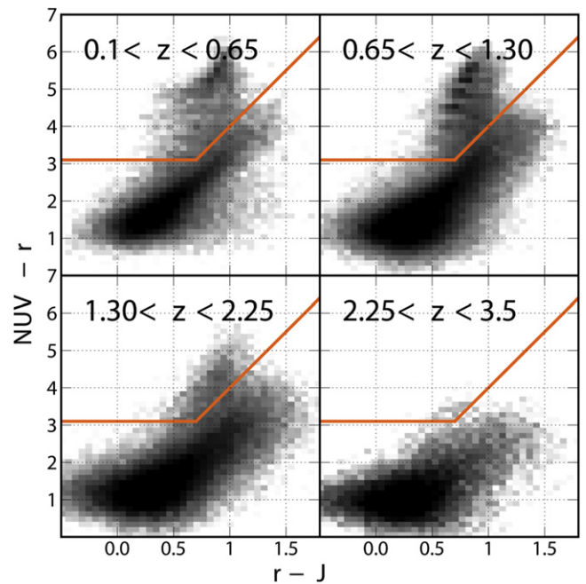
Figure 16. NUV - r/r - J galaxy distributions. Quiescent galaxies lie in the top-left corner. The objects fainter than limiting magnitudes are not used.
