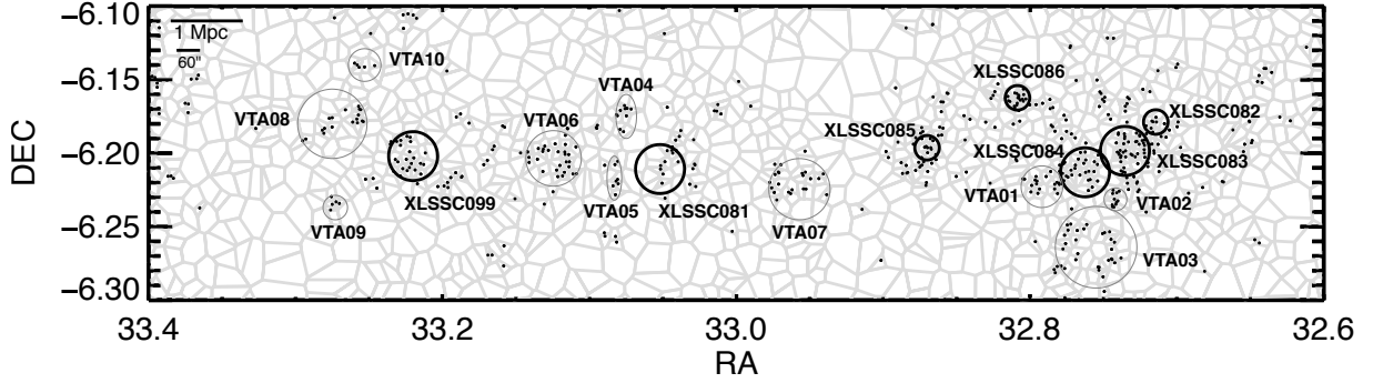
Fig. 7. Voronoi tessellation analysis of the area around the X-ray identified cluster structure at 0.35 < z_{\text{phot}} < 0.50 (lines). Galaxies associated with overdense structures identified via our VTA analysis (see text for details) are shown as black dots. A projected scale of 1 Mpc is indicated in the top left corner. The X-ray identified clusters are marked with thick black circles, and VTA identified overdense structures are marked with thin grey circles. Galaxies within these regions were sampled to statistically estimate the properties of clusters and overdense structures. (See Table 3 for details.)
