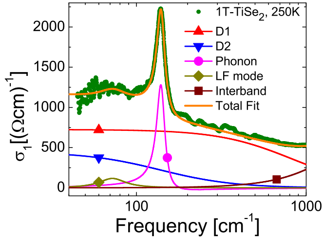
FIG. 3. The real part of the optical conductivity of 1T -TiSe _2 below 1000\text{ cm}^{-1} at 250\text{ K} along with the decomposition into components as discussed in the text. The related decomposition for the imaginary part is provided in the Supplemental Material [48].
