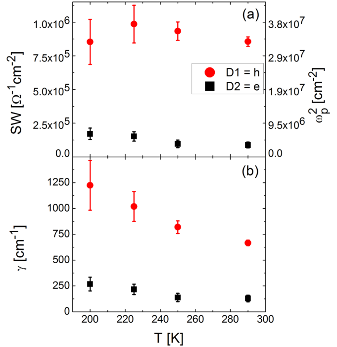
FIG. 4. The results of the Kramers-Kronig-consistent fit to the experimental optical data of 1T -TiSe 2 in the high-temperature phase ( 290\text{ K} \geq T \geq 200\text{ K} ). (a) Spectral weights of two Drude terms that model the electronic response below 1000\text{ cm}^{-1} . SW is the spectral weight of the Drude term defined as SW = \pi \varepsilon_0 \omega_p^2 / 2 , where \omega_p is the plasma frequency. The right axis shows the square of the plasma frequency. (b) The quantity \gamma is the width (or damping) of the Drude term expressed in \text{cm}^{-1} , inversely proportional to the transport scattering time.
