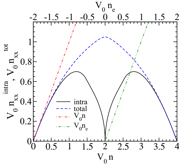
FIG. 3. The effective numbers of charge carriers n_{\alpha\alpha}^{intra}(\mathbf{q}) and n_{\alpha\alpha}^{tot}(\mathbf{q}) calculated by using Eq. (26), for n_L(\mathbf{k}) = f_L(\mathbf{k}) , t = 2.52 eV, T = 100 K, and \mathbf{q} \approx \mathbf{0} . V_0 n = (1/N) \sum_{Lk\sigma} f_L(\mathbf{k}) is the concentration of conduction electrons ( V_0 n = 2 in pristine graphene) and V_0 is the primitive cell volume.
