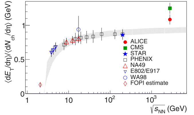
FIG. 12. Comparison of \langle dE_T/d\eta \rangle / \langle dN_{\text{ch}}/d\eta \rangle at midrapidity versus \sqrt{s_{NN}} in Pb-Pb collisions at \sqrt{s_{NN}} = 2.76 TeV from ALICE and measurements at other energies [19,23,25,26,29,64,67]. The band shows the extrapolation from lower energies with the width representing the uncertainty on the fit [26].
