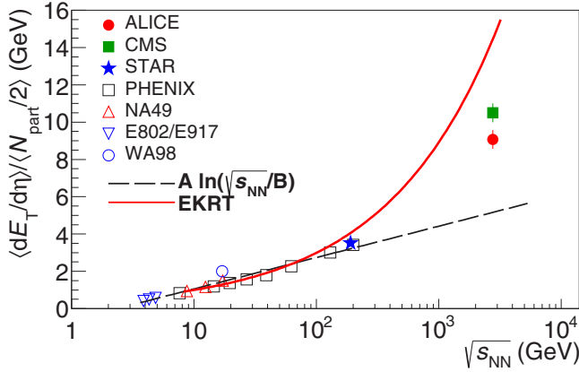
FIG. 11. Comparison of \langle dE_T/d\eta \rangle / \langle N_{\text{part}}/2 \rangle at midrapidity versus \sqrt{s_{NN}} in 0%–5% central Pb-Pb collisions at \sqrt{s_{NN}} = 2.76 TeV from ALICE and CMS [30] and central collisions at other energies [26,29,64] at midrapidity. All measurements are from 0%–5% central collisions except the NA49 data, which are from 0%–7% collisions.
