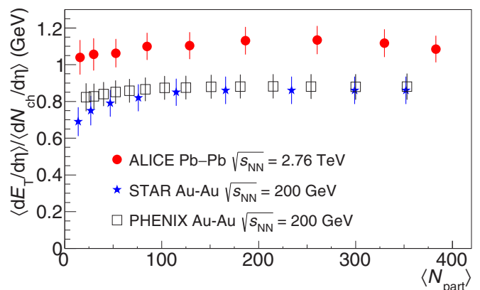
FIG. 10. Comparison of \langle dE_T/d\eta \rangle / \langle dN_{\text{ch}}/d\eta \rangle versus \langle N_{\text{part}} \rangle at midrapidity in Pb-Pb collisions at \sqrt{s_{NN}} = 2.76 TeV from ALICE and in Au-Au collisions at \sqrt{s_{NN}} = 200 GeV from STAR [29] and PHENIX [26,27].
