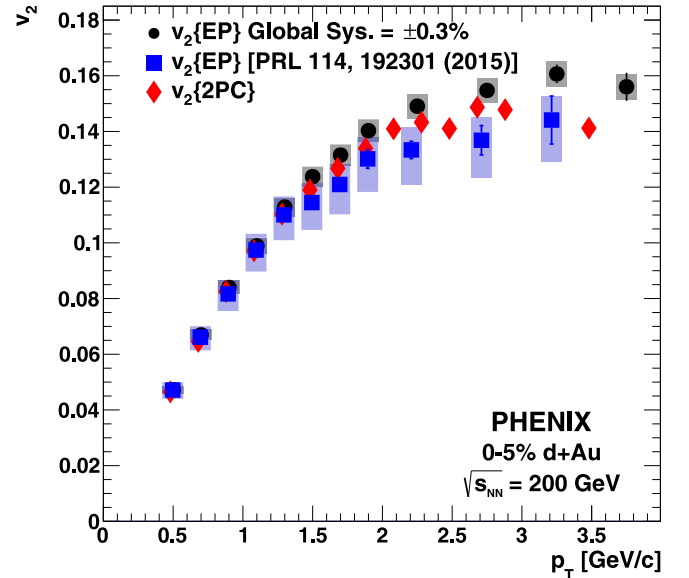
FIG. 4. The v_2 vs. p_T in 0%–5% central d + \text{Au} collisions at \sqrt{s_{NN}} = 200 GeV using the event-plane method (black filled circles) and two-particle correlations (red filled diamonds). Also shown are the previously published v_2 vs. p_T using the event-plane method (blue filled squares) from PHENIX using data collected in 2008 [15].
