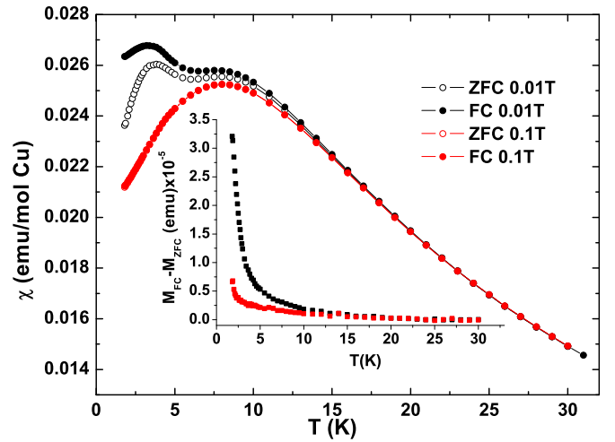
FIG. 3. Low-field susceptibility measurement on an unoriented powder sample. In the magnetic field of 0.01 T, FC and ZFC susceptibility start to differ at 15 K. Upon increasing magnetic field this difference vanishes. Inset show differences between FC and ZFC magnetization curves in a field of 0.01 T (black) and 0.1 T (red).
