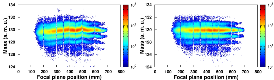
Fig. 3. Matrices of Te mass ( Z = 52 ) versus focal plane position before (left) and after (right) the empirical corrections described in the text.
