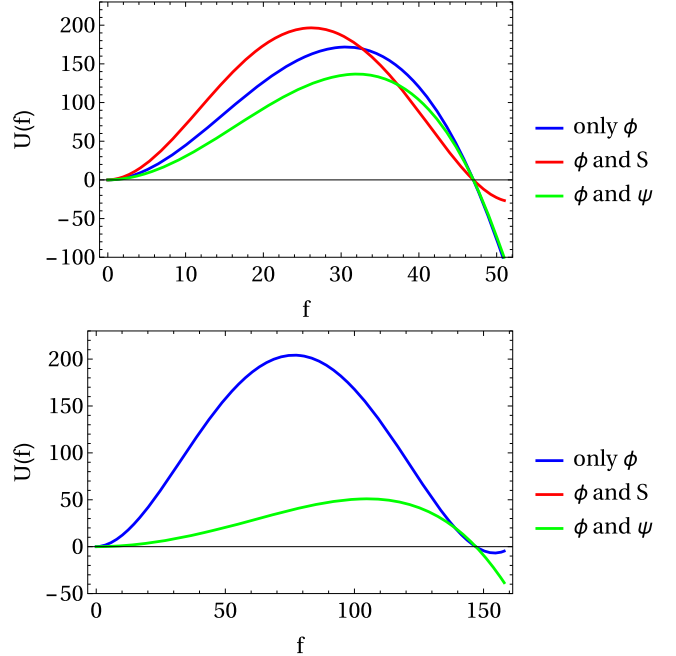
Fig. 3. Reduced potential U(f) which a final state bubble has to tunnel through. Upper panel: f_f = 47 , lower panel: f_f = 147 . Without new physics in blue, and with new physics scalar S in red and with fermion \psi in green. Note that the stabilizing effect of the scalar S has shut down the decay channel to an f_f = 147 bubble. (For interpretation of the references to color in this figure, the reader is referred to the web version of this article.)
