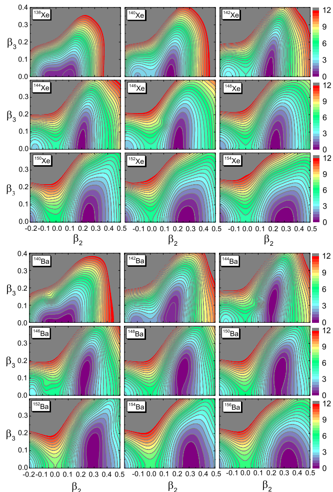
FIG. 6. Deformation energy surfaces of ^{138-154}\text{Xe} and ^{140-156}\text{Ba} in the \beta_2 - \beta_3 deformation plane, calculated with the RMF+BCS model using the PC-PK1 functional and \delta -force pairing.
