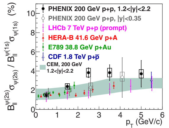
FIG. 3. Comparison of world data on the ratio of \psi(2S)/\psi(1S) mesons as a function of p_T [29,40,43–45], along with a calculation from a color evaporation model (CEM) at \sqrt{s} = 200 \text{ GeV} [25].
