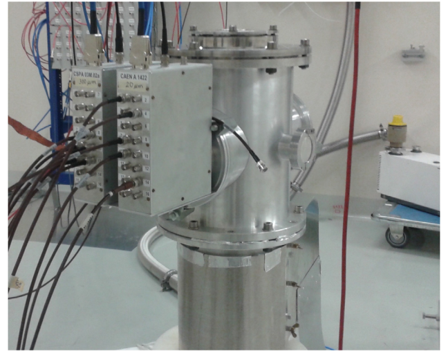
Fig. 3. The scattering chamber, with the front-end electronics, installed on the vertical neutron beam line in EAR2. The target and the telescope detector are inside.
