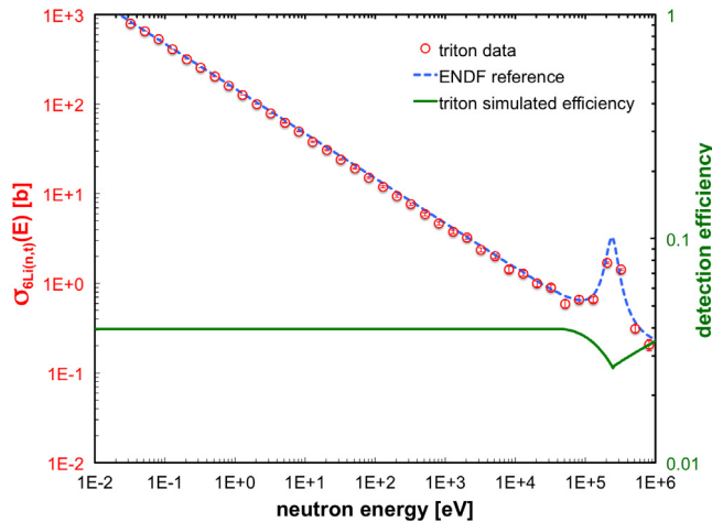
Fig. 9. The {}^6\text{Li}(n,\alpha)t cross-section (circles), as measured during the validation test, is in good agreement with the international standard (dashed line) and thus can be used for normalization. The green continuous line, to be read on the right-hand axis, represents the triton detection efficiency as simulated by means of GEANT4.
