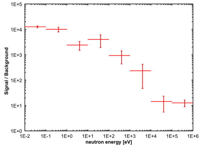
Fig. 15. The signal-to-background ratio in eight neutron energy bins. The signal was the number of proton events in the ^7\text{Be}(n,p)^7\text{Li} reaction. The background data were produced using a dummy target with only the aluminum backing.
