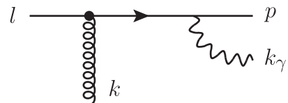
FIG. 1. Example for a LO diagram for photon production in the high-energy limit. The blob contains multiple (eikonal) scatterings on the dense target with momentum exchange k . The complete LO contribution includes photon emission before the interaction with the nucleus (not shown).
