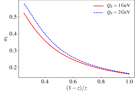
FIG. 5. a_1 for g \rightarrow q\gamma to order Q_\perp^2/\tilde{P}_\perp^2 as a function of the photon isolation cut for the MV model with two different saturation scales. We take Q_\perp/\tilde{P}_\perp = 0.1 , \tilde{P}_\perp = 15Q_S and \zeta = 1 .
