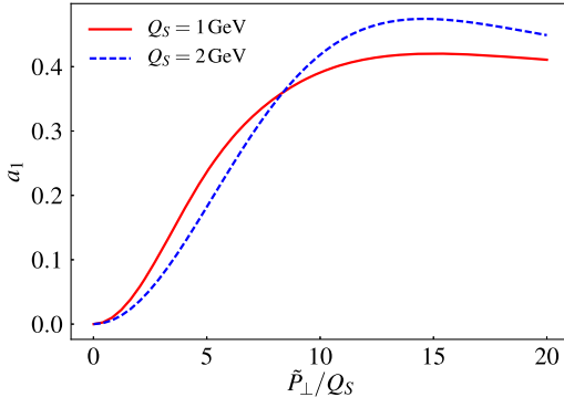
FIG. 3. a_1 for g \rightarrow q\gamma to order Q_\perp^2/\tilde{P}_\perp^2 for the MV model with two different saturation scales. We take Q_\perp/\tilde{P}_\perp = 0.1 , z = 3/4 and \zeta = 1 .
