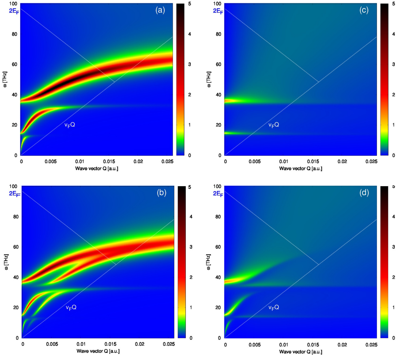
FIG. 5. The spectra of surface excitations in (a) graphene (200 meV)/SiO 2 single slab (as shown in Fig. 2), (b) in the system consisting of two equal graphene (200 meV)/SiO 2 slabs, (as shown in Fig. 1) separated by distance 5 nm, (c) single graphene (0 meV)/SiO 2 slab, and (d) in the system consisting of two unequal slabs, graphene (200 meV)/SiO 2 and graphene (0 meV)/SiO 2 , separated by distance 5 nm.
