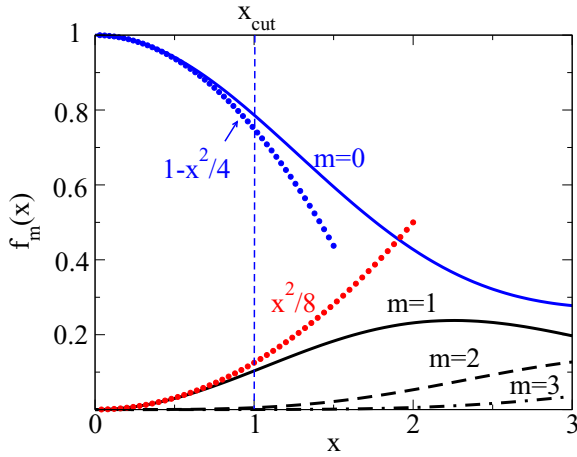
FIG. 4. Function f_m(x) for m = 0 (blue solid line), m = 1 (black solid line), m = 2 (black dashed line), and m = 3 (black dashed-dotted line). Vertical dashed line denotes the maximum argument x_{cut} defined by parameters ( a and \rho_0 ) used in the calculation.
