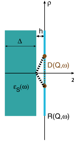
FIG. 2. Simplified model where the SiO 2 substrate is shown as a homogenous dielectric slab described by the local dielectric function \epsilon_S(\omega) and graphene is described by 2D response function R(\mathbf{Q}, \omega) . D(\mathbf{Q}, \omega) is the surface excitation propagator of the substrate/graphene composite.
