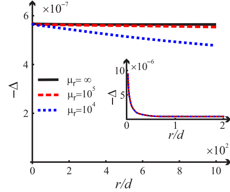
FIG. 2. Parameter -\Delta = -e\pi^{-1}\hbar^{-1} \oint \mathbf{A} \cdot d\mathbf{l} as a function r/d , for three values of \mu_r ; d = 10 nm (see text for details).
