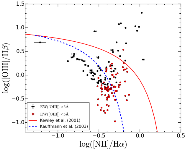
Fig. 15. BPT diagram for radio sources in XXL-S. The red points are those for which EW([O\ III]) < 5\ \text{\AA} , and the black points are those for which EW([O\ III]) > 5\ \text{\AA} . The error bars were calculated according to Eqs. (13) and (14). The solid red line is the extreme starburst line from Kewley et al. (2001) and the dashed blue line is the star-forming galaxy line from Kauffmann et al. (2003).
