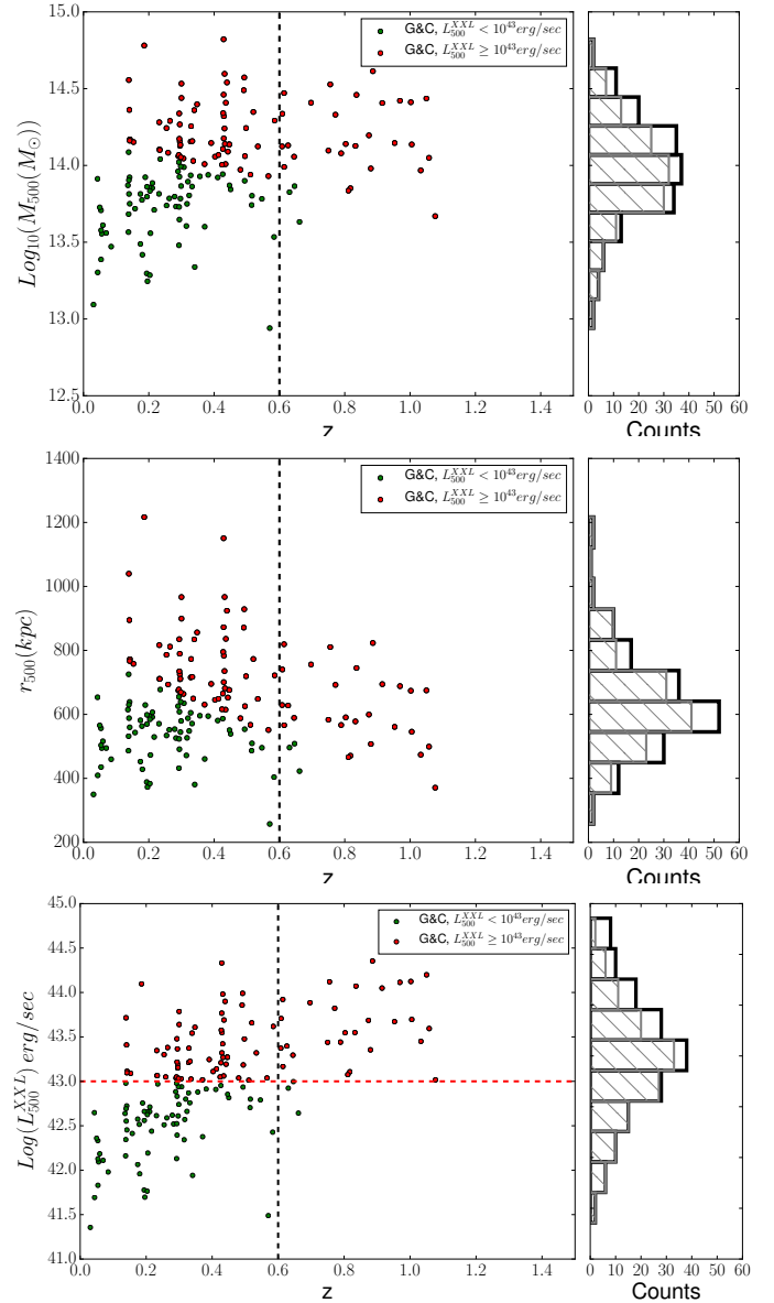
Fig. 2. Main panels: M_{500,scal} (upper), r_{500,scal} (middle), L_{500,scal}^{XXL} (bottom) vs. redshift for the 164 XXL-N c1+c2 G&C with estimates of M_{500,scal} and r_{500,scal} . The distribution of the same quantities is shown in the corresponding right panels, where black histograms refer to all G&C in the sample, and grey hatched histograms are for z \leq 0.6 G&C. In the main panels, the vertical black dashed line corresponds to z = 0.6 , the maximum redshift of G&C considered in this work. High-luminosity G&C are marked in red, low-luminosity G&C in green. In the bottom panel, the horizontal red dashed line corresponds to the luminosity used to separate the G&C into two classes (see text for details).
