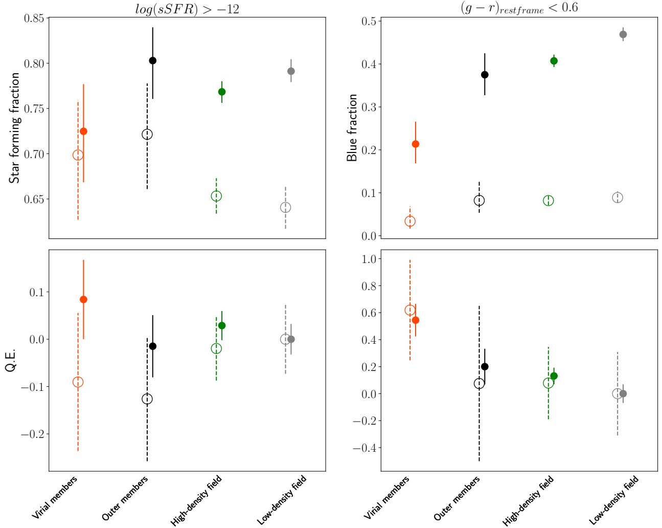
Fig. 6. Fraction of star-forming galaxies in different environments, computed with sSFR (left panel) and rest-frame colour (right panel). The fractions obtained using the magnitude-limited sample are represented with filled symbols and solid errors, those obtained using the mass-limited sample are represented by empty symbols and dashed error bars. Errors are derived by means of a bootstrap method. The two lower panels show the quenching efficiency (Q.E.) in different environments, computed with Eq. (3) for both the star-forming and blue samples. The Q.E. of field galaxies, which is by definition set to zero (see Eq. (3)), is shown in both panels as a reference. The error bars on the Q.E. of the low-density field depend on the amplitude of the confidence intervals associated with the fractions of star-forming and passive galaxies from bootstrapping.
