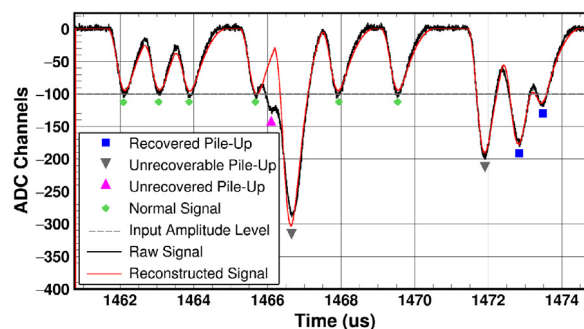
Fig. 2. Typical signal reconstruction recorded at 1 MHz. Apart from the raw and the reconstructed signals, different pile-up cases which are marked with symbols, are shown. See text for further details.
