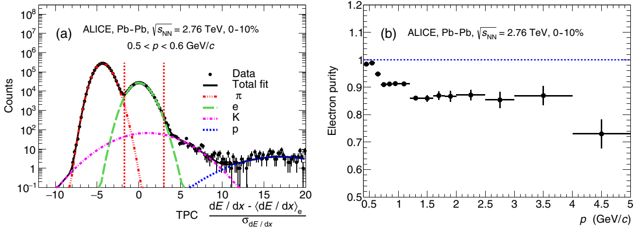
FIG. 1. (a) Distributions of the difference between the measured dE/dx in the TPC and the expected average value for electrons (in units of \sigma_{TPC} ) after the selection of the electron candidates in the TOF ( |n\sigma_{TOF}(e)| < 3 ) and in the ITS ( -5 < n\sigma_{ITS}(e) < 1 ). (b) Electron purity as a function of the track momentum ( p ) estimated from the multiple skewed Gaussian fit.
