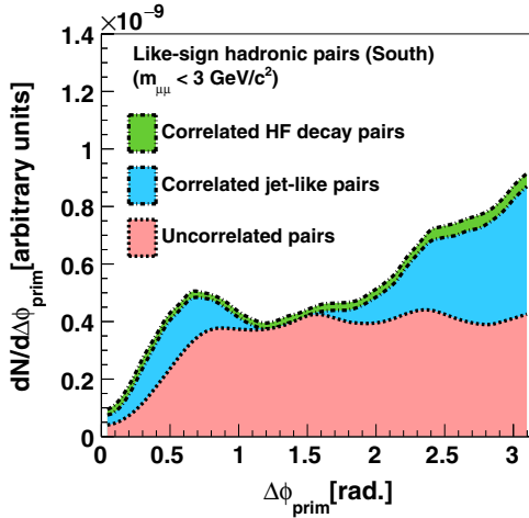
FIG. 11. ZYAM normalization procedure for the south muon arm. The normalization of the unrelated pairs from event mixing (red) is determined by enforcing the requirement that the yield of the unrelated pairs ( N_{\text{corr, sim}} ) is identical to the yield of foreground pairs ( N_{hb} ), excluding the pairs from heavy-flavor decay chains (green) at \Delta\phi_{\text{prim}} \sim \pi/2 . The excess yield is from away-side and near-side jetlike correlations (blue). The periodicity of the distributions arises from the octant structure of the MuTr.
