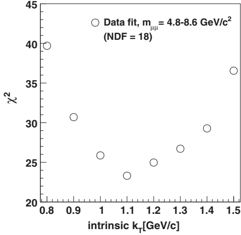
FIG. 21. The \chi^2 for the pair p_T spectrum of Drell-Yan pairs in the mass region 4.8–8.6 GeV/ c^2 compared to PYTHIA simulations with different intrinsic k_T . The \chi^2 is minimized at a k_T of 1.1 GeV/ c .
