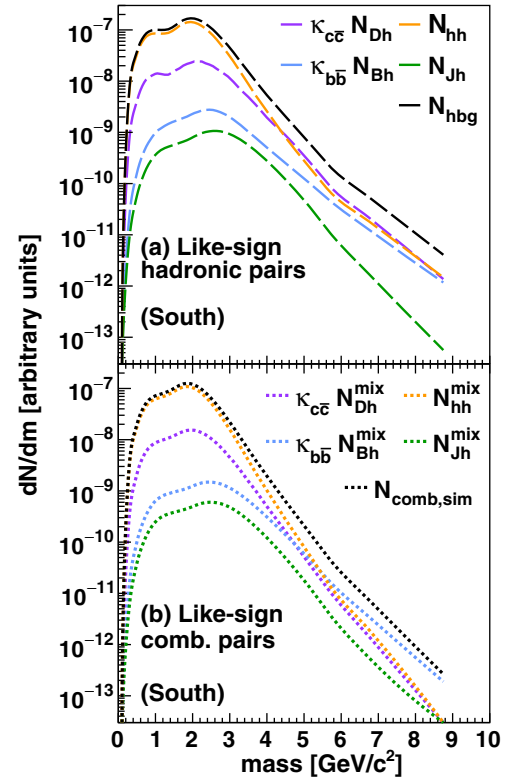
FIG. 10. (a) full simulation for hadronic pairs and (b) combinatorial pairs for mass spectra of hadron-hadron and muon-hadron pairs from charm, bottom and J/\psi after initial normalization and tuning.
