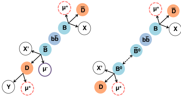
FIG. 1. Like-sign muon pairs from bottom decays arise from a combination of B \rightarrow \mu and B \rightarrow D \rightarrow \mu decay chains or from decays following B^0\bar{B}^0 oscillations.
