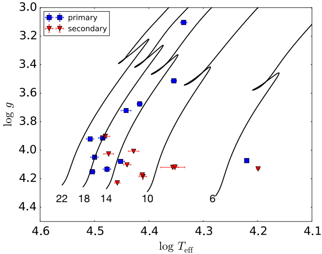
Fig. 1. Positions of individual binary components from our sample in Table 1 in the T_{\text{eff}}-\log g Kiel diagram. Blue squares and red triangles refer to the primary and secondary components, respectively. Evolutionary tracks are computed with solar metallicity Z = 0.014 and for an exponentially decaying CBM profile with f_{\text{ov}} = 0.02 H_p . Stellar mass is indicated in M_{\odot} units.
