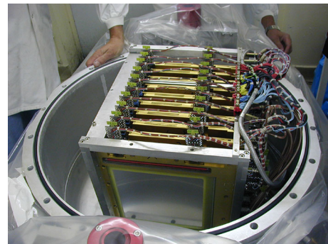
Fig. 14 The experimental setup with PPAC and actinide samples, assembled for Phase-I at n_TOF. Ten detectors and nine samples are mounted inside a vacuum chamber perpendicular to the neutron beam
