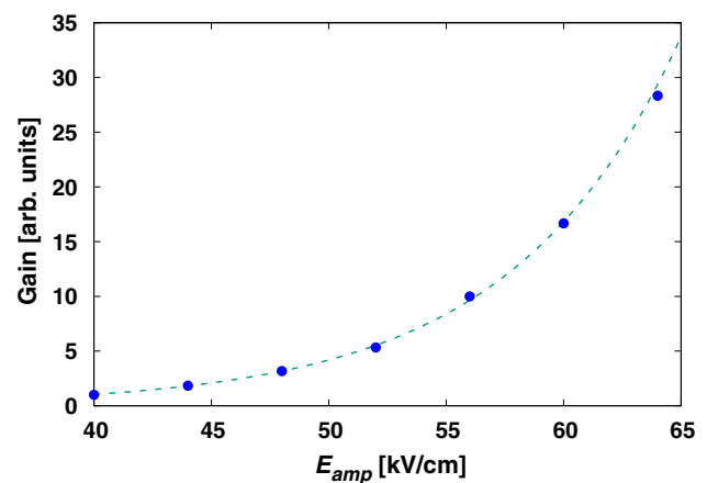
Fig. 22 A typical gain curve obtained with a Micromegas detector with a 50 \mu\text{m} amplification gap filled with an \text{Ar}:\text{CF}_4:\text{isoC}_4\text{H}_{10} gas mixture, with the voltage applied to the cathode kept constant at 600 V. The gain (here arbitrarily set equal to 1 for an electrical field in the amplification region E_{\text{amp}}=40\text{ kV/cm} ) changes exponentially with the electrical field strength E_{\text{amp}} (an exponential fit of the data points is shown, dashed line). Typical values of the absolute gain are between 10^3 and 10^5 [135]
