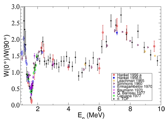
Fig. 56 Energy dependence of the FFAD of ^{232}\text{Th} , measured with the PPAC system (tilted configuration), compared to previous measurements (see Ref. [209])
