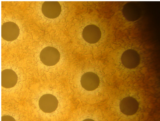
Fig. 19 A photograph of a micromesh obtained with a digital microscope from a Micromegas detector used at n_TOF. The holes have a diameter of 40\ \mu\text{m} and are distributed in a triangular pattern with a 100\ \mu\text{m} pitch. (Courtesy: A. Teixeira, CERN)
