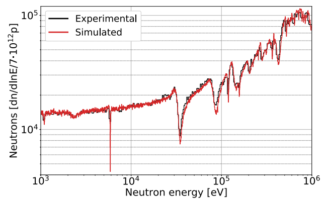
Fig. 41 A comparison of the evaluated neutron energy distribution for EAR-1 (measured with the small collimator) and the simulated distribution for the same setup
