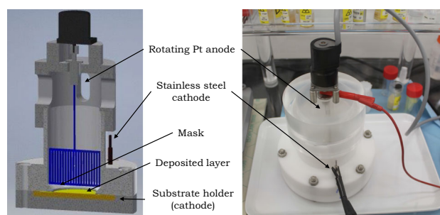
Fig. 33 Cross section (left) and picture (right) of a molecular plating cell to prepare actinide deposits at JRC-Geel
