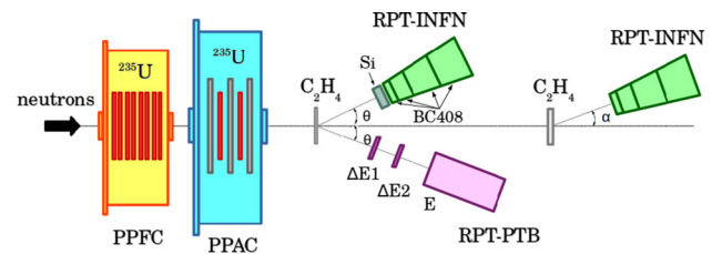
Fig. 30 Drawing of the setup used at n_TOF for the quasi-absolute measurement of the ^{235}\text{U}(\text{n},\text{f}) cross section. Fission reactions are measured with a fission chamber and a set of Parallel Plate Avalanche Counters (described in Sect. 4.2). Recoil protons are detected and identified in three different telescopes (two of which of identical design), placed at a small angle outside the neutron beam. Polyethylene and pure carbon samples of various thickness are used in the measurement
