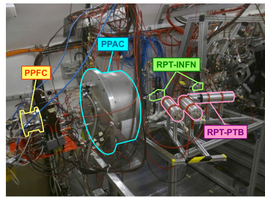
Fig. 31 Photo of the experimental setup used at n_TOF for the quasi-absolute measurement of the ^{235}\text{U}(\text{n}, \text{f}) cross section from 20 MeV to 1 GeV. The setup was mounted in the neutron beam-line of the first experimental area
