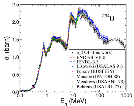
Fig. 51 The ^{234}\text{U}(n,f) cross section measured with the PPAC setup (perpendicular configuration), above the fission threshold [69]. High-accuracy data have been obtained for the first time up to 1 GeV neutron energy
