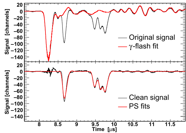
Fig. 36 Example of signals recorded with a micromegas detector operated at low gain, typically used for fission measurements, exhibiting a consistent response to the initial \gamma -flash. The top panel shows the average \gamma -flash-induced distortion adjusted to the actual signal. The bottom panel shows the signal corrected for this distortion and being subjected to the separate pulse-shape fitting
