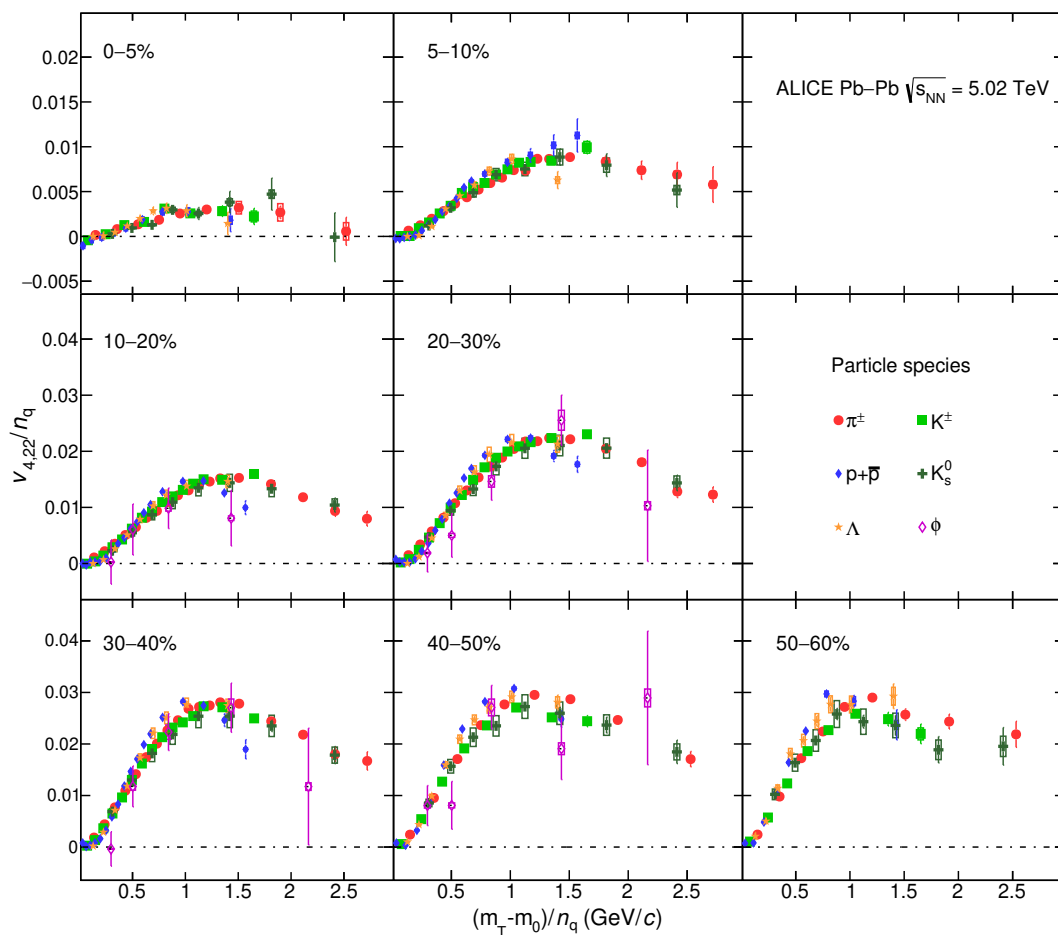
Figure 22. The (m_T - m_0)/n_q -dependence of v_{4,22}/n_q for different particle species grouped into different centrality intervals of Pb-Pb collisions \sqrt{s_{NN}} = 5.02 TeV. Statistical and systematic uncertainties are shown as bars and boxes, respectively. It is seen that the KE_T scaling holds for v_{4,22} at an approximate level.
