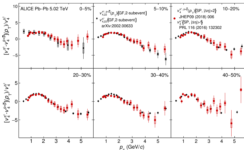
Figure 14. The comparison between [v_{4,22}^{\pi^\pm} - v_4^{p+\bar{p}}](p_T)/v_4^{h^\pm} and [v_4^{\pi^\pm} - v_4^{p+\bar{p}}](p_T)/v_4^{h^\pm} grouped into different centrality intervals of Pb-Pb collisions at \sqrt{s_{NN}} = 5.02 TeV. Statistical and systematic uncertainties are shown as bars and boxes, respectively.
