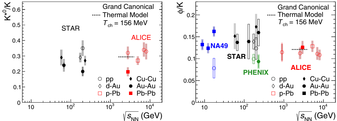
FIG. 5. Particle ratios of K^{*0}/K (left) and \phi/K (right) are presented for pp , high-multiplicity p -Pb, central d -Au, and central A -A collisions [10–13,28–31,33–41] as a function of the collision energy. Bars (when present) represent statistical uncertainties. Boxes represent the total systematic uncertainties or the total uncertainties for cases when separate statistical uncertainties were not reported. The value given by a grand-canonical thermal model with a chemical freeze-out temperature of 156 MeV [27] is also shown.
