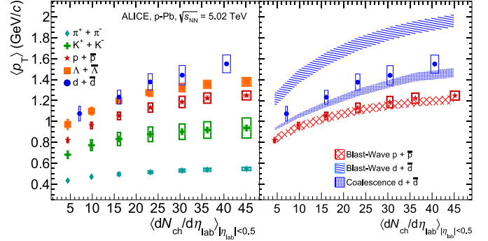
Fig. 8. Mean p_T of various particle species as a function of the mean charged-particle density at mid-rapidity for different V0A multiplicity classes. The empty boxes show the total systematic uncertainty while the shaded boxes indicate the contribution which is uncorrelated across multiplicity intervals (left). Comparison of \langle p_T \rangle of protons and deuterons with the simple coalescence and the Blast-Wave model expectations. The shaded areas show the expected \langle p_T \rangle for deuterons from a simple coalescence model assuming a p_T -independent B_2 as well as the calculated \langle p_T \rangle for protons and deuterons from the Blast-Wave model [43] using the kinetic freeze-out parameters for pions, kaons, protons and \Lambda from [18] (right).
