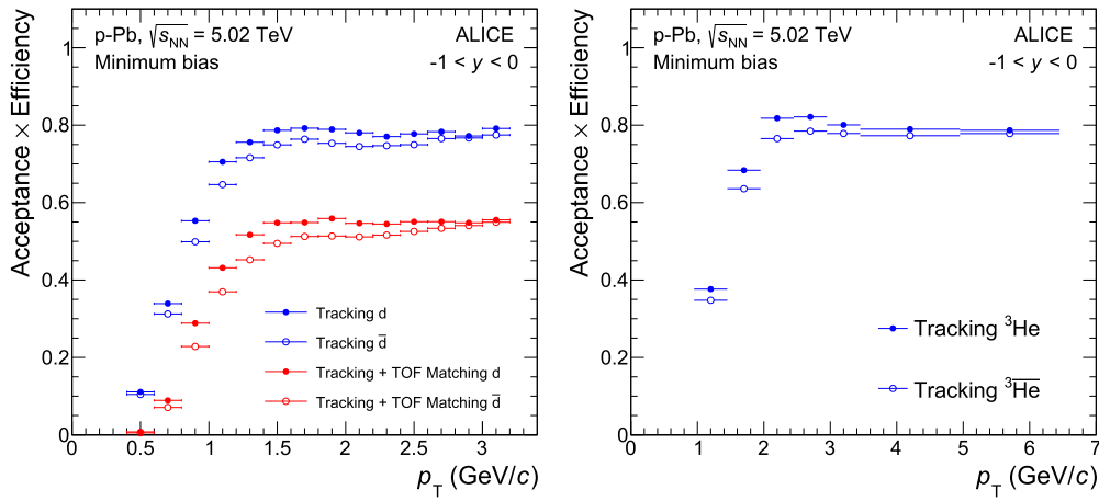
Fig. 2. Tracking acceptance \times efficiency correction for (anti-)deuterons (left) and for ^3\text{He} and ^3\bar{\text{He}} (right) in the minimum-bias class. The efficiencies for anti-nuclei are lower due to the larger cross-section for hadronic interactions.
