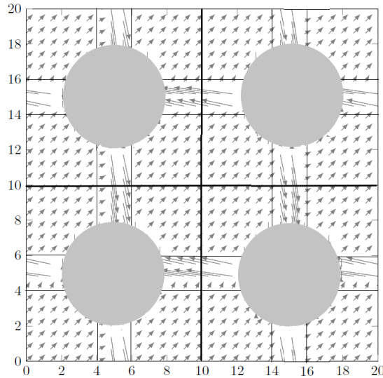
Figure 4.3: Representation of vector field b out side of supp \sigma
