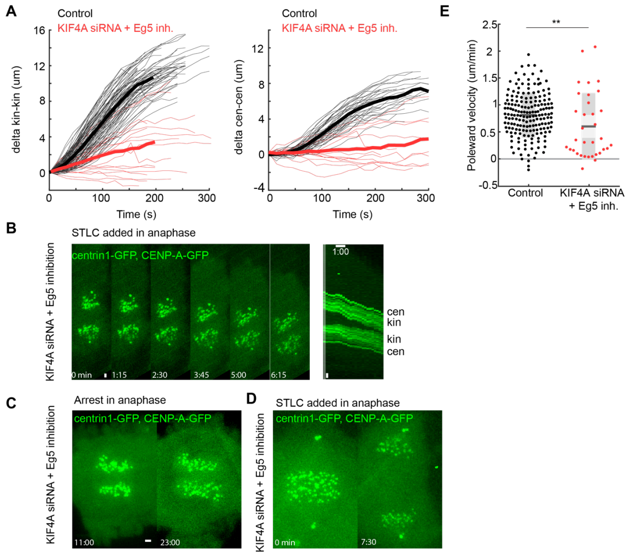
Figure 41. Depletion of KIF4A combined with EG5 inhibition blocks spindle elongation in anaphase. (A) Plots of relative kinetochore and centrosome separation distance ( \Delta ) defined as the kinetochore-to-kinetochore (kin-kin) and centrosome-to-centrosome (cen-cen) distance at time t minus the kin-kin and cen-cen distance at t = 0 , over time in KIF4A siRNA depleted and S-trityl-L-cysteine (STLC)-treated RPE-1 cells stably expressing CENP-A-GFP and centrin1-GFP. Individual kinetochore and centrosome pairs (thin lines), mean (thick lines). (B) Live cell images of a cell from (A) show perturbed spindle elongation when STLC is added in anaphase. kin-kinetochore and cen-centrosome. (C) Live cell images of KIF4A siRNA depleted and STLC-treated RPE-1 cell show long-term anaphase arrest phenotype when STLC is added in anaphase. (D) Live cell images of KIF4A siRNA depleted and STLC-treated RPE-1 cell, with addition of STLC in anaphase, show small rate of spindle elongation. Note: in few examples, if STLC was added in early anaphase, spindle elongation could be observed but to lesser degree when compared to controls. Time 0 represents start of STLC treatment. (E) Quantification (univariate scatter plot) of kinetochore to pole velocities
