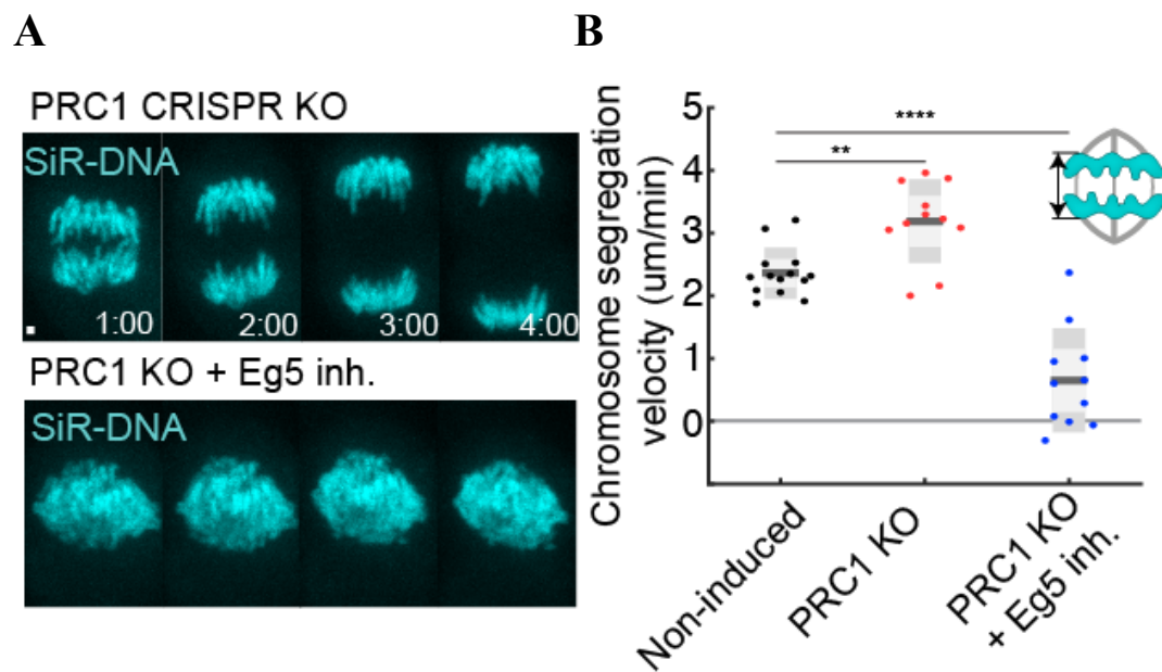
Figure 37. Loss of PRC1 and inactivation of EG5 blocks spindle elongation during anaphase. (A) Live cell images of induced RPE-1 PRC1 CRISPR knock-out (KO) and PRC1 KO treated with STL. Silicon rhodamine (SiR)-DNA was used for chromosome staining. (B) Quantification of chromosome segregation velocity (see scheme) in CRISPR experiments. Statistics: t test (**P < 0.01; ****P < 0.0001). Images are maximum projection of acquired z-stack. Time 0 represents anaphase onset. Scale bar, 1 μm.
