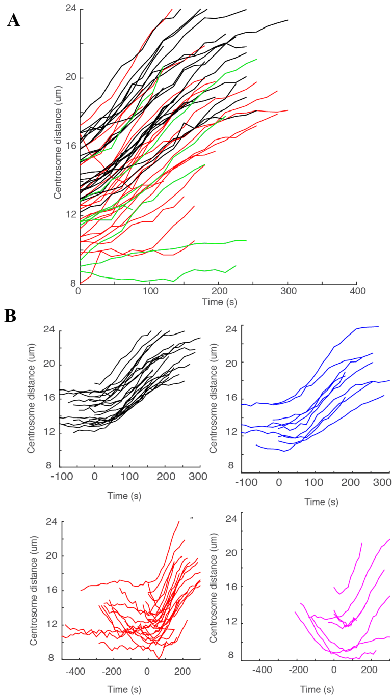
Figure 23. Inhibition of STLC, with or without combined depletion of KIF15, is dispensable for anaphase spindle elongation. (A) Centrosome distance plotted as a function of time where zero represent onset of centrosome separation. Black lines indicate control cells, red lines indicate STLC-treated cells and green lines indicate KIF15-depleted cells combined with inhibition of EG5 by STLC. (B) Centrosome distance plotted as a function of time where zero represent onset of kinetochore separation. Black lines; control cells, red lines;
