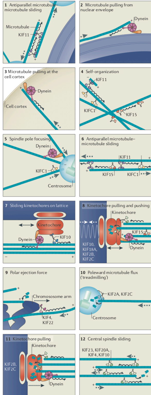
Figure 8. Functional roles of motor proteins in mitosis of human cell. Proposed involvement of multiple mitotic motors in the key mitotic processes noted on the left with some key mechanisms distinguished and numbered on the right incorporating all stages of mitosis. See details through the text. Taken from Cross and McAinsh, 2014.
