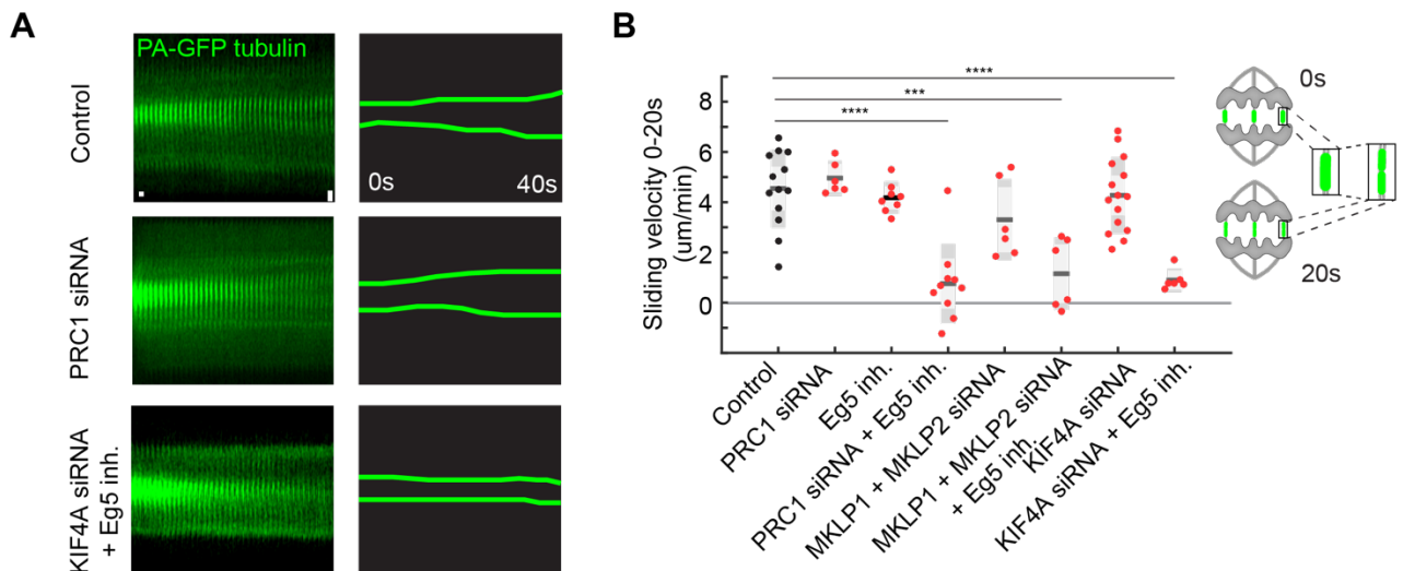
Figure 57. Chromosome segregation and spindle elongation are dependent upon KIF4A and EG5-generated sliding. (A) Montage time-lapse live images of mitotic spindle midzone region after photoactivation of photoactivatable (PA)-GFP- \alpha -tubulin in indicated treatments. Note that photoactivated spot does not spread in time after KIF4A siRNA depletion and STLC
