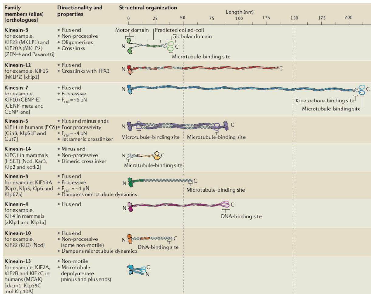
Figure 7. Mitotic kinesin motors. Representation of mitotic kinesins in human cells with list of various nomenclatures used, alternative names and ortologues from other organisms together with directionality information, note about important properties and structural organization illustrations with the main domains depicted. See details through the text. Taken from Cross and McAinsh, 2014.
