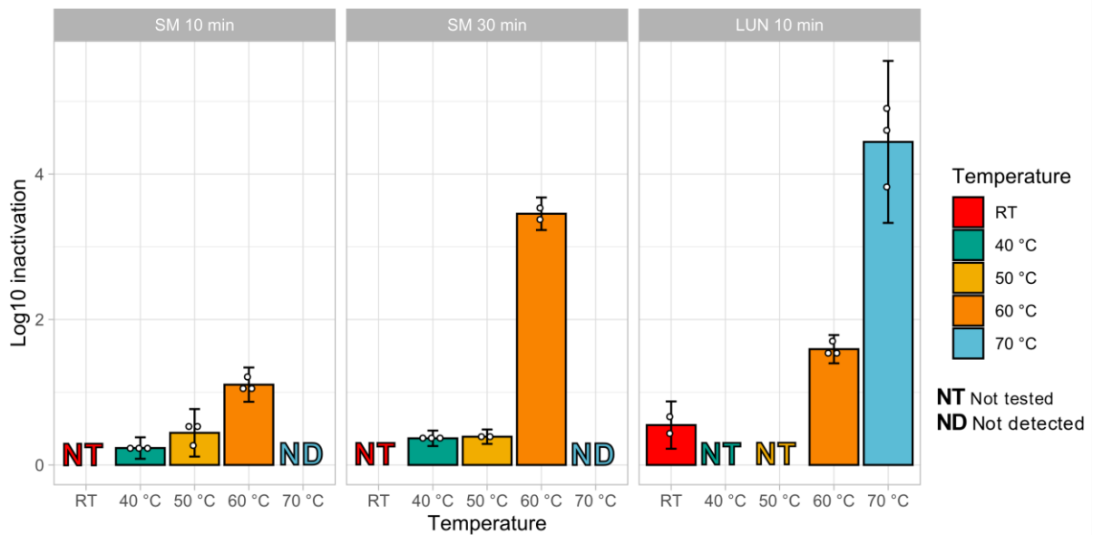
Figure 3.5. Loss of MS2 phage infectivity after treatment for 10 and 30 min at room temperature (RT), 40, 50, 60 and 70 °C. Phages were treated in SM buffer ( SM 10 min and SM 30 min ) and lunar dust simulant ( LUN 10 min ). Error bars represent SD (n = 2 or 3).
