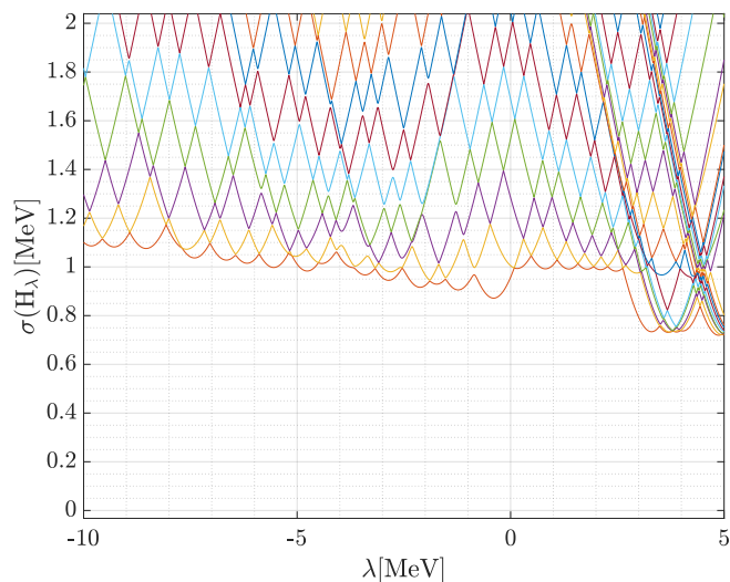
Figure 2.3: Same as Figure 2.2 only zoomed in. Closer inspection suggest that distinct eigenvalues indeed do not cross each other as they evolve with changing the parameter \lambda .
