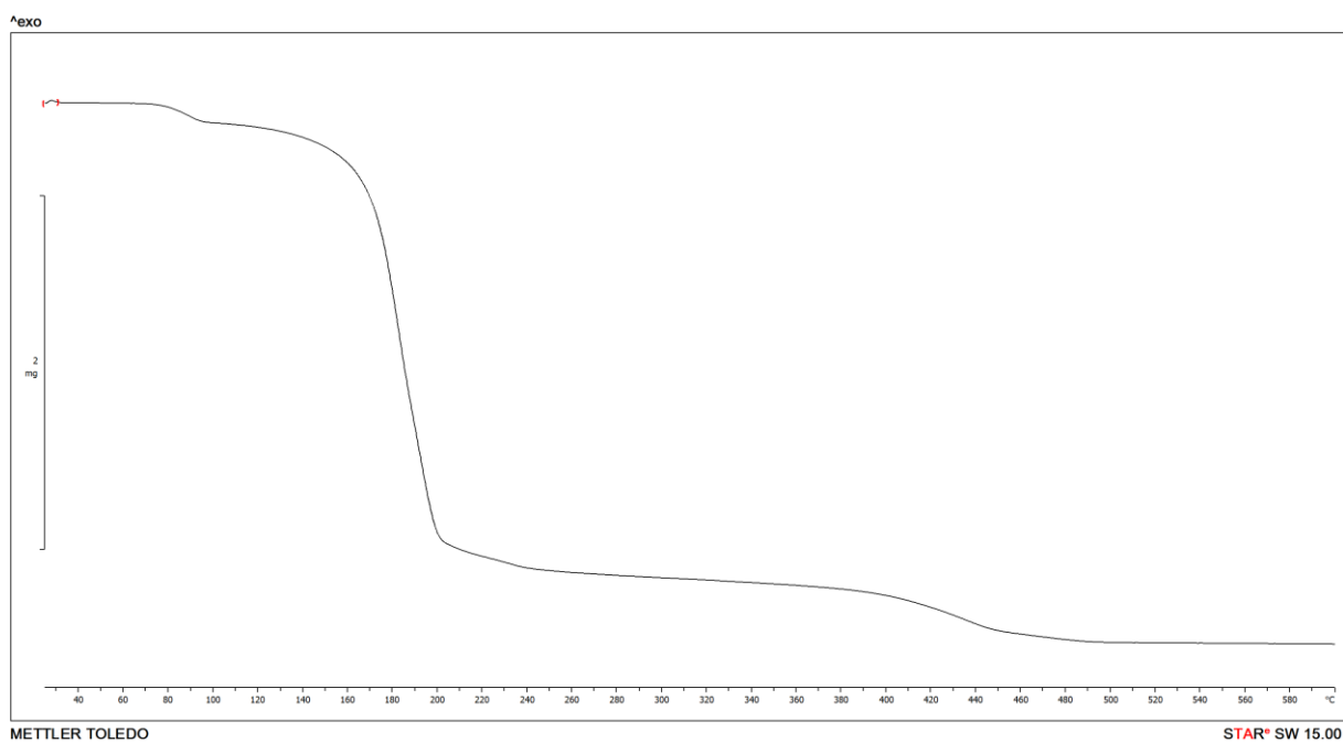
Slika D44. TG krivulja kokristala soli [\text{Ni}(\text{H}_2\text{O})_2(\text{Acpy})_2]\text{Cl}_2 \cdot 14\text{H}_2\text{O} .
