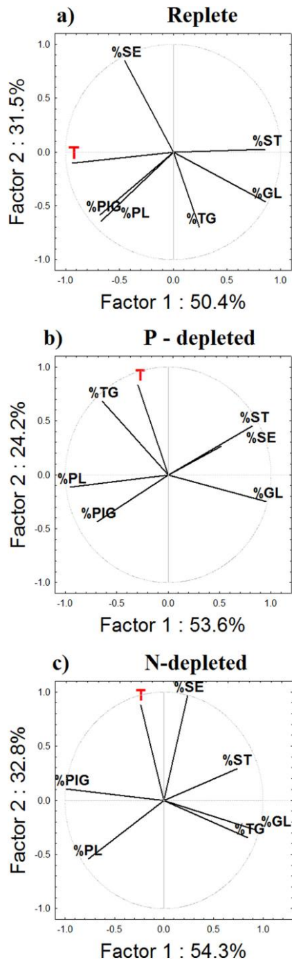
Fig. 4. Principal component analysis (PCA) for the variables: temperature (T), contribution of different lipid classes to total cell lipids: triacylglycerol (%TG), sterol ester (%SE), sterol (%ST), pigment (%PIG), phospholipid (%PL), and glycolipid (%GL) at replete (a), P-depleted (b) and N-depleted (c) growth conditions.
