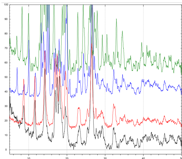
Slika 21. Usporedba difraktograma prahova kompleksa reakcijom s \text{H}_2\text{4OHSal-4HBOH} ligandom u metanolu: [\text{MoO}_2(4\text{OHSal-4HBOH})(\text{H}_2\text{O})] (metoda A; crveno), [\text{MoO}_2(4\text{OHSal-4HBOH})(\text{H}_2\text{O})] \cdot \text{MeOH} (metoda B; plavo), [\text{MoO}_2(4\text{OHSal-4HBOH})(\text{H}_2\text{O})] (metoda C; crno) i metoda D (zeleno).
